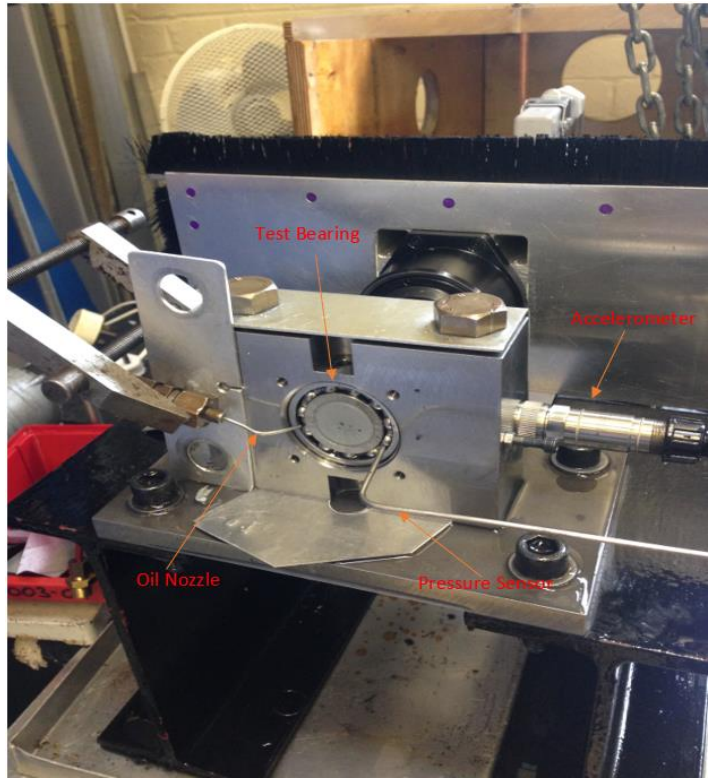
Windage test rig
