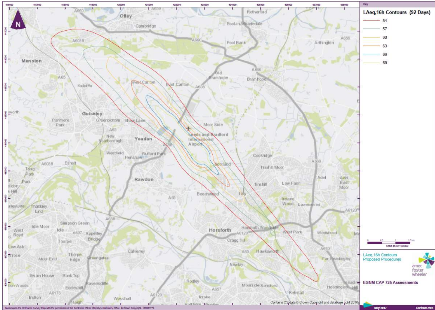
Figure 13 - Noise Contours for Existing Traffic Levels with New Procedures.
