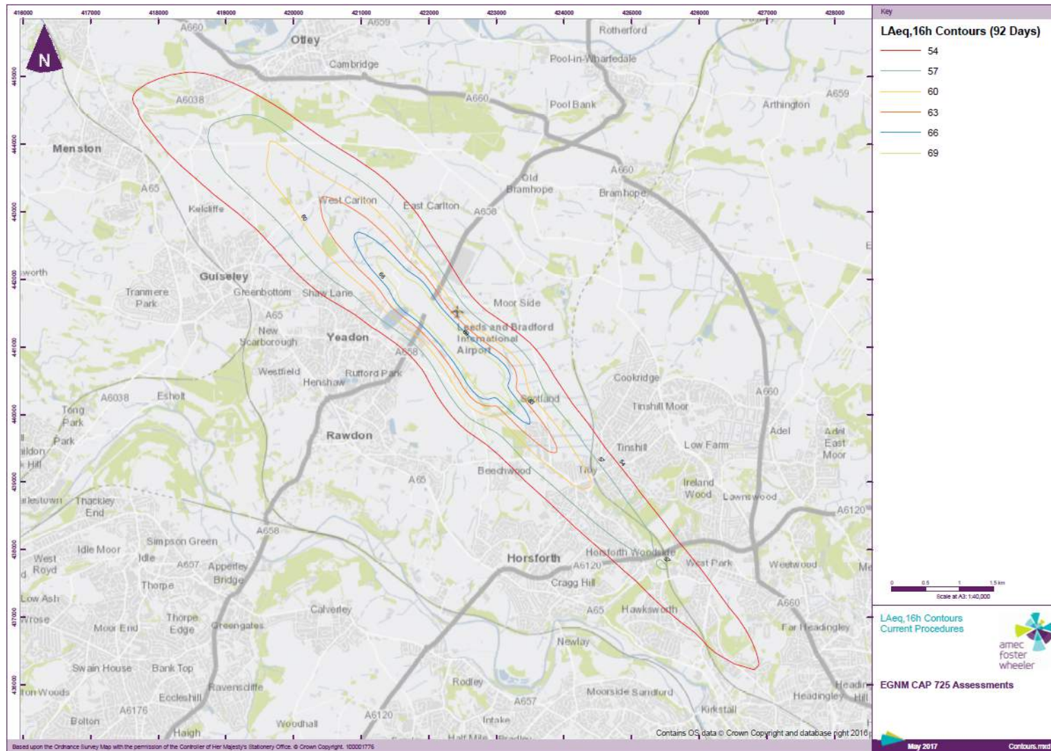
Figure 12 - Noise Contours for Existing Traffic Levels.
