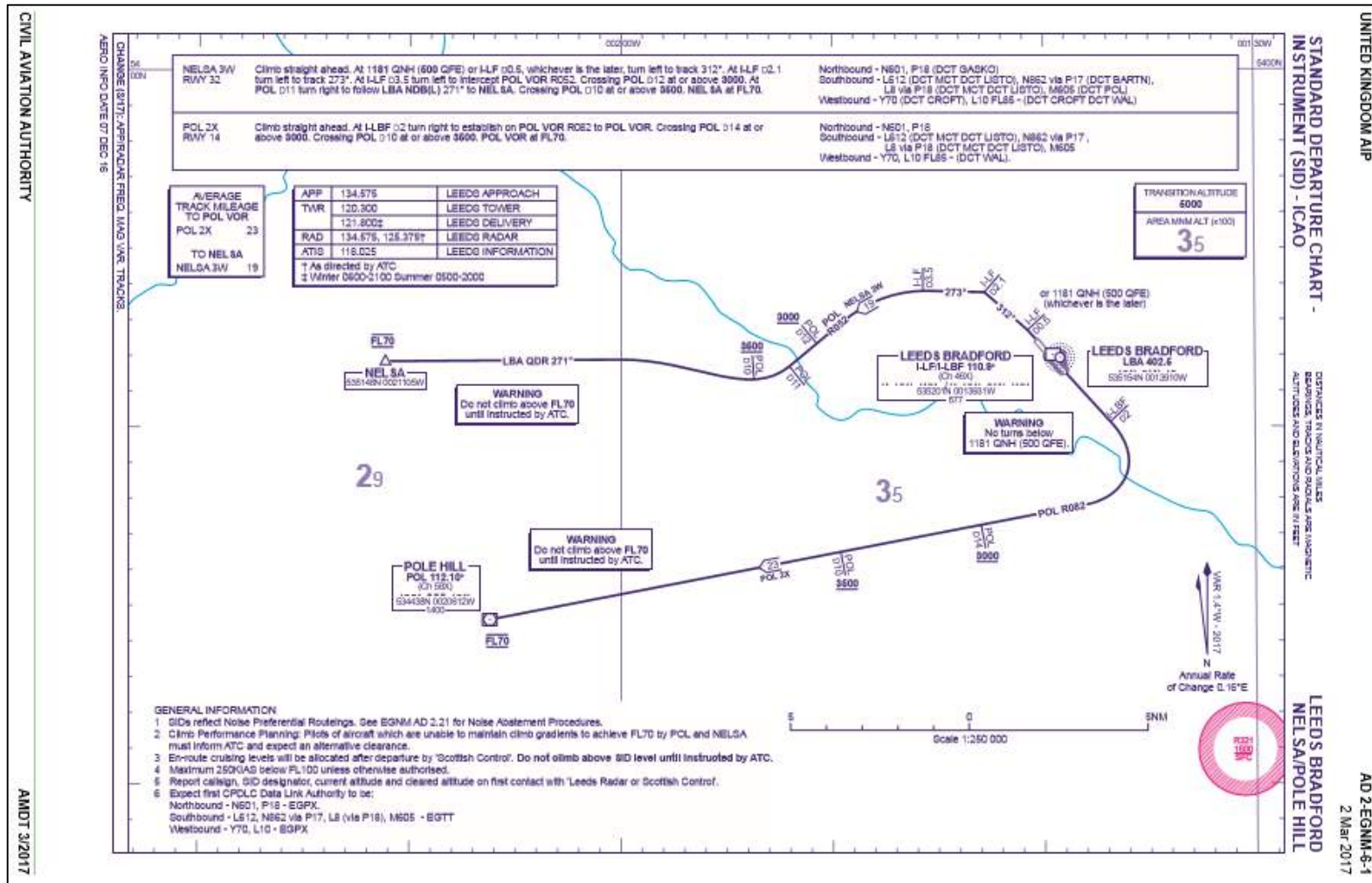
Figure 2. Current Standard Instrument Departures – NELSA/POLE HILL (Available at http://www.ead.eurocontrol.int/eadbasic/pamslight-0EA5010DC20CC86C50175510792BC9F9/7FE5QZZF3FXUS/EN/Charts/AD/AIRAC/EG_AD_2_EGNM_6-1_en_2017-03-02.pdf )
