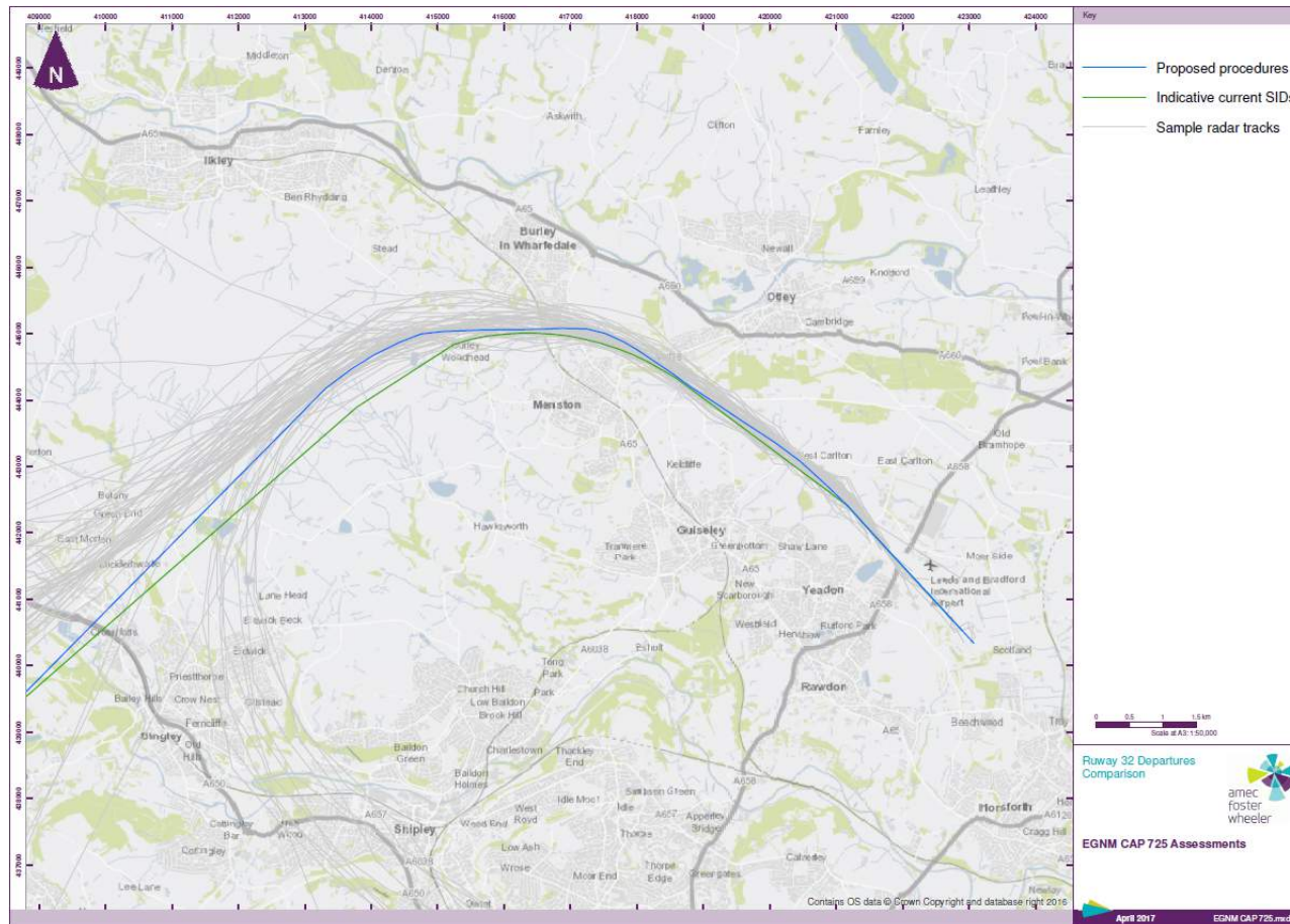
Proposed Procedures vs Sample Radar Tracks for Runway 32.
