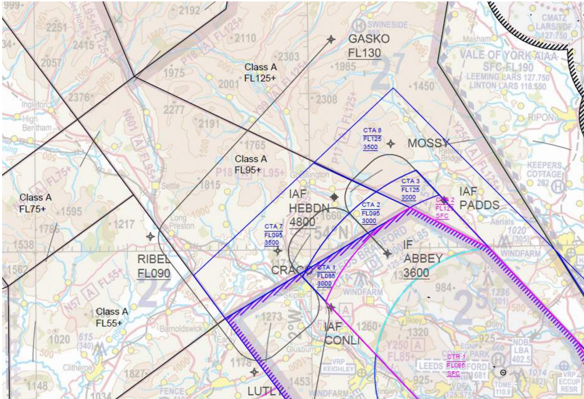
Figure 8. Draft Arrival Routes from the North to Runway 14
