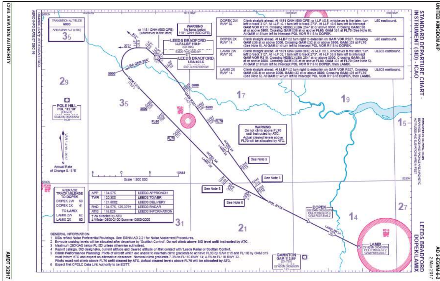
Figure 1. Current Standard Instrument Departures – DOPEK/LAMIX (Available at http://www.ead.eurocontrol.int/eadbasic/pamslight-OEA5010DC20CC86C50175510792BC9F9/7FE5QZZF3FXUS/EN/Charts/AD/AIRAC/EG_AD_2_EGNM_6-2_en_2017-03-02.pdf )
