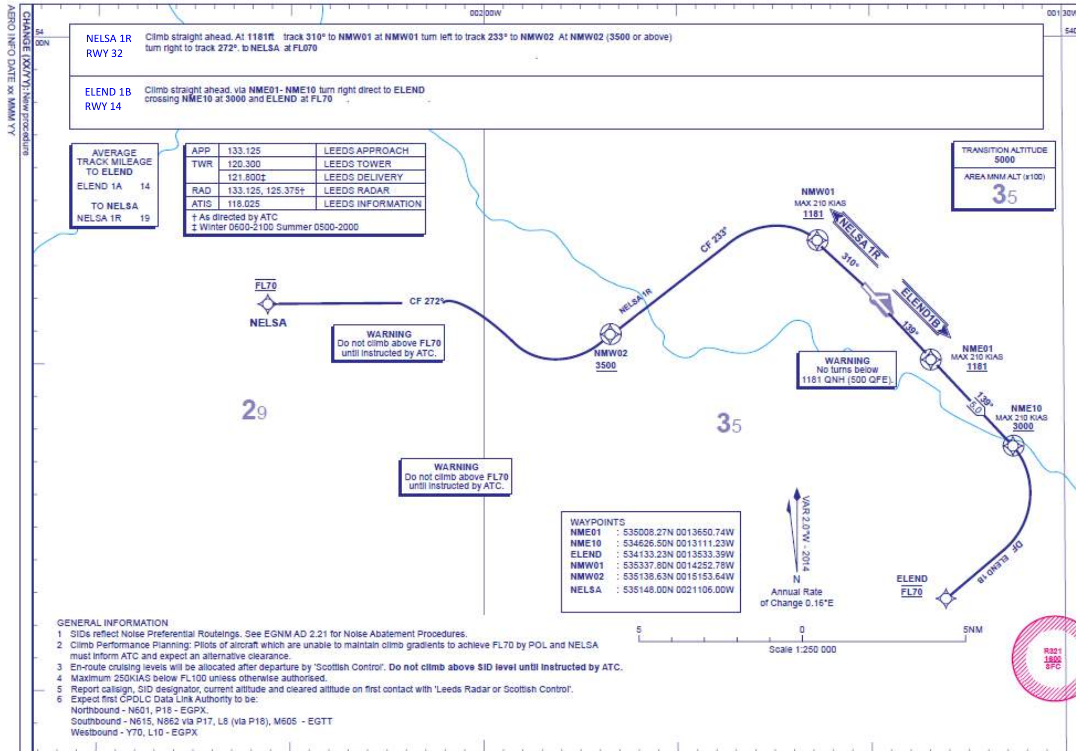
Figure 5. Draft GNS Standard Instrument Departures – NELSA/ELEND
