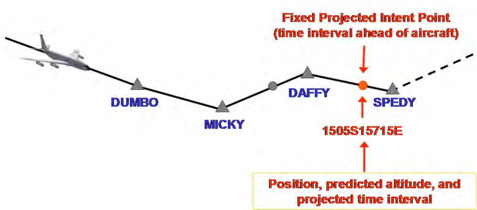
Figure 2-45. ADS-C fixed projected intent group
