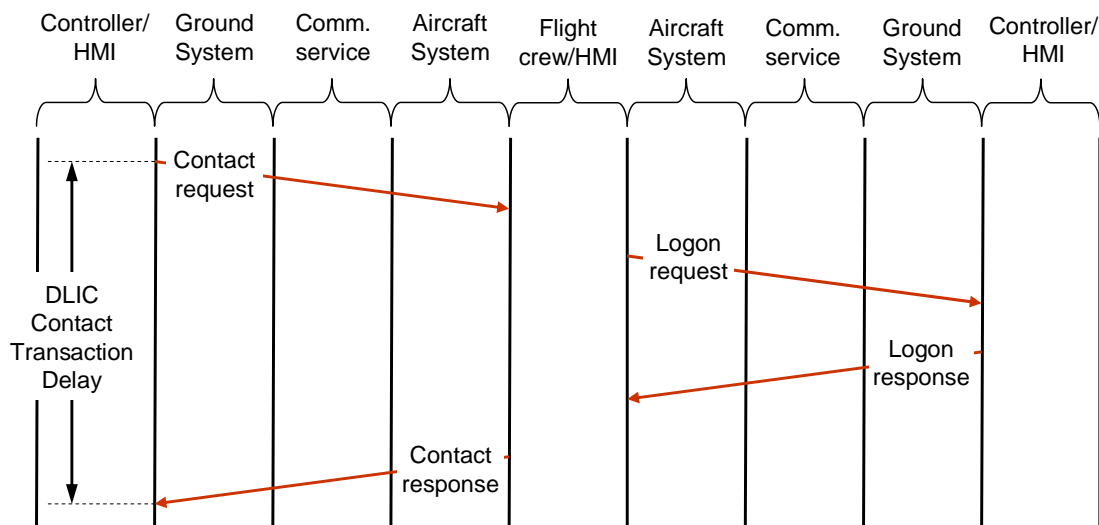
Figure D-5 DLIC Contact transaction
